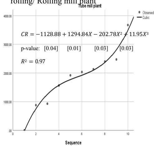
Figure 5: Physical Deterioration of Tube mill plant
